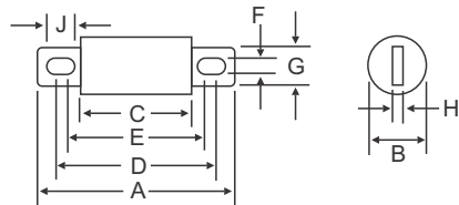
Diagram 1 (35A - 1200A)
