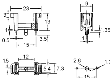
Mounting Pattern
