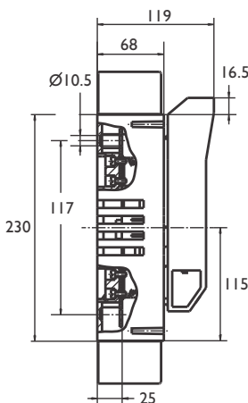
Battery Fuse 550VDC Size I (p65)
