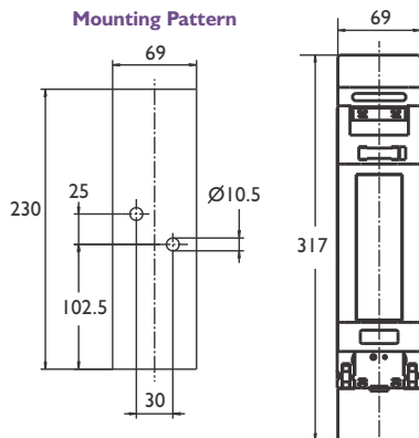
Mounting Pattern
