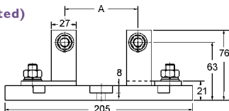
Diagram 2 (1250A Rated)
