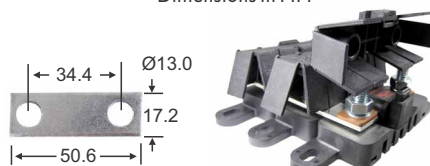
2 Hole Bus Bar
